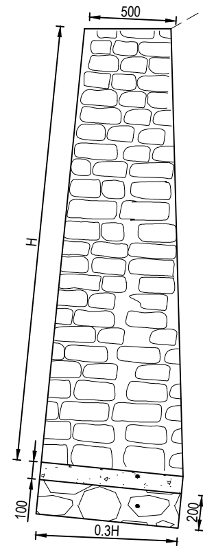
Typical Section of Masonry Breast wall Scale 1:30
