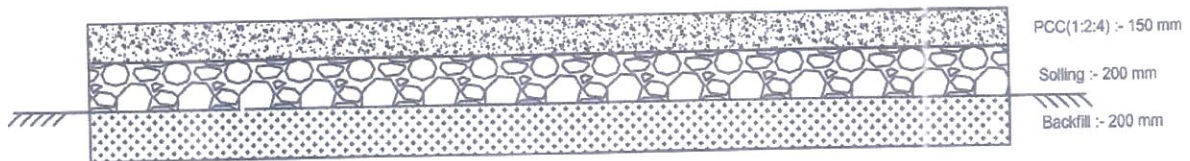
SOLLING With PCC CROSS SECTION
