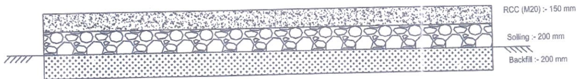
SOLLING With RCC/CAUSE WAY CROSS SECTION
