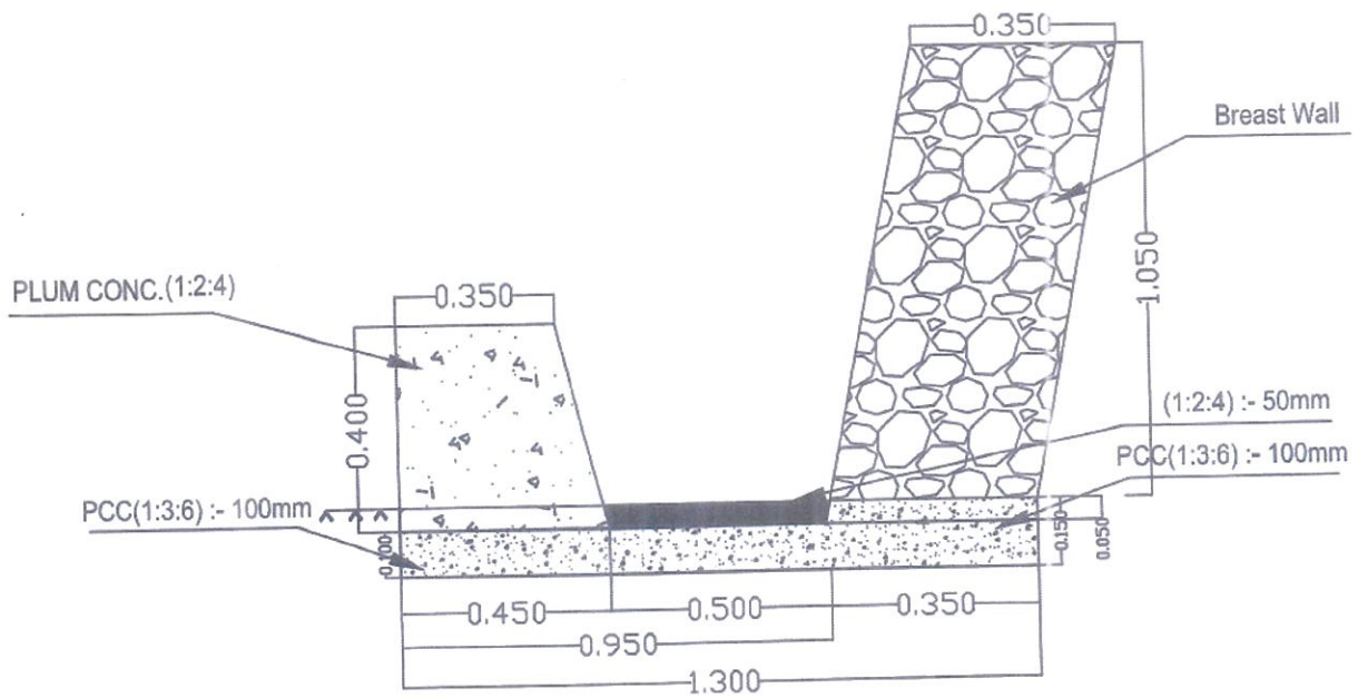
DRAIN CROSS SECTION. (-typical)
