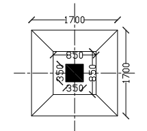
Footing plan Type F1, 1.7mX1.7m
