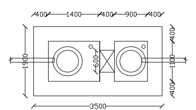
PLAN septic tank 2.3mx1.1m [20users for 2 years]
