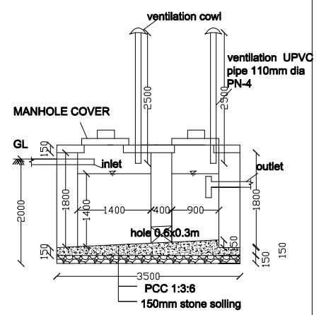
SECTION septic tank 2.3mx1.1m [20users for 2 years]
