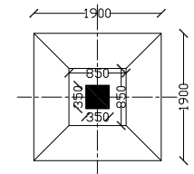
Footing plan Type F2, 1.9mX1.9m
