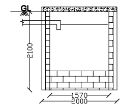
SECTION SOCKPIT
