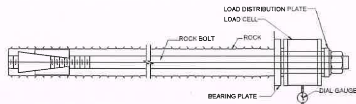
TYPICAL LOAD CELL
