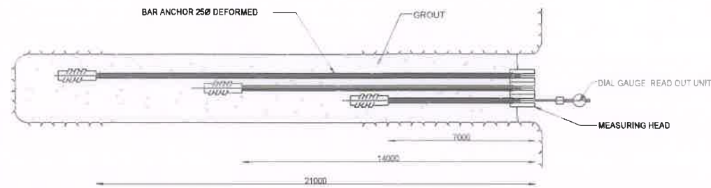
TYPICAL MULTI-POINT BOREHOLE EXTENSOMETER (MPBX)
