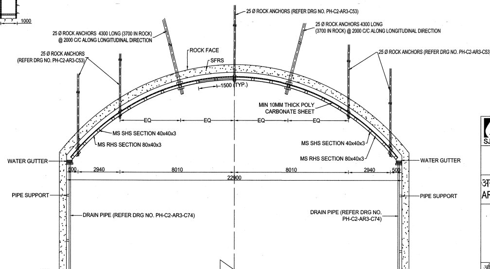
SECTION A-A X-SECTION OF FALSE CEILING
