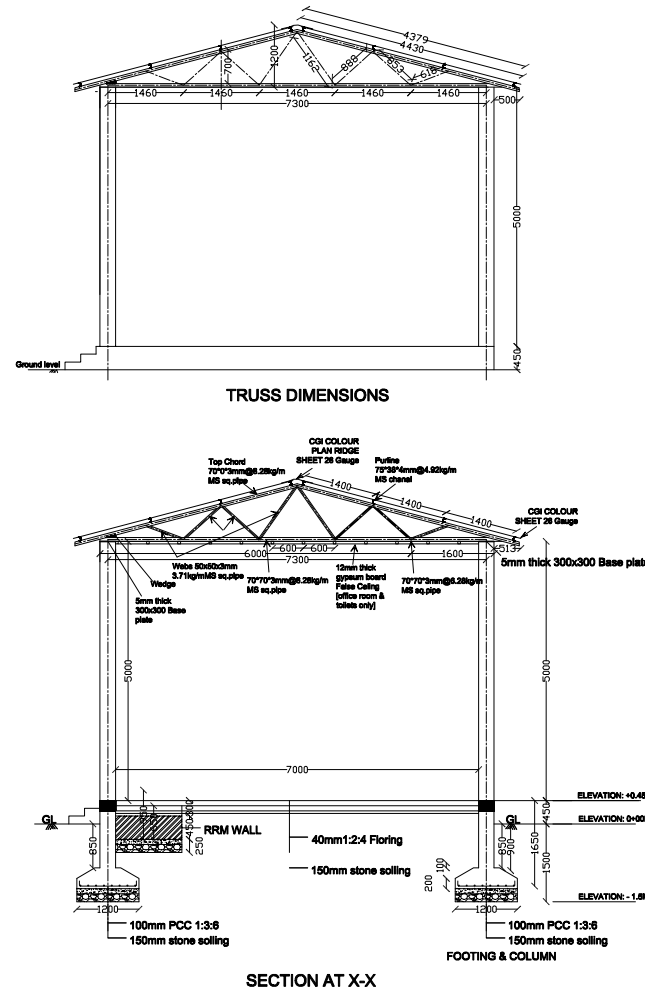
SECTION AT X-X
