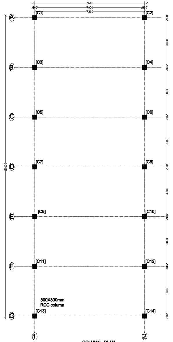
COLUMN PLAN
