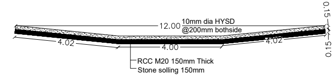
Causway section Rd-0+886 to 0+892 [12mX6mX.15m]
